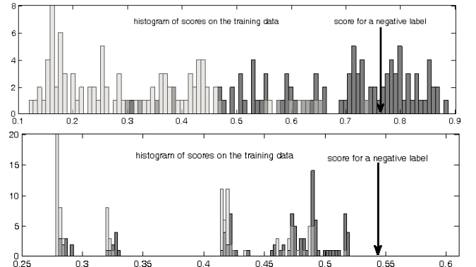
Figure 4. Histogram of anomaly scores for 2 different tasks. The scores for the top and bottom task range from 0.1 to 0.9 and from 0.25 and 0.61, respectively. The arrow in both cases points to the scores of the evaluated examples, both with negative labels. Despite the score is lower for the bottom task, we may believe that it is more anomalous because it is more extreme within the scores for the same task.
