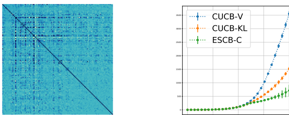
Figure 2: Left: Correlation matrix of the dataset, right: Cumulative regret, averaged over 36 independent simulations
