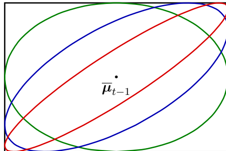
Figure 1: Confidence regions build by ESCB-C (the pseudo-ellipse), and CUCB-KL (the rectangle), for \|\cdot\|_1 constrained outcomes. Notice that CUCB-KL has slightly better confidence intervals along the axis, but that ESCB-C is better in the direction \mathbf{e}_{\{1,2\}} .
