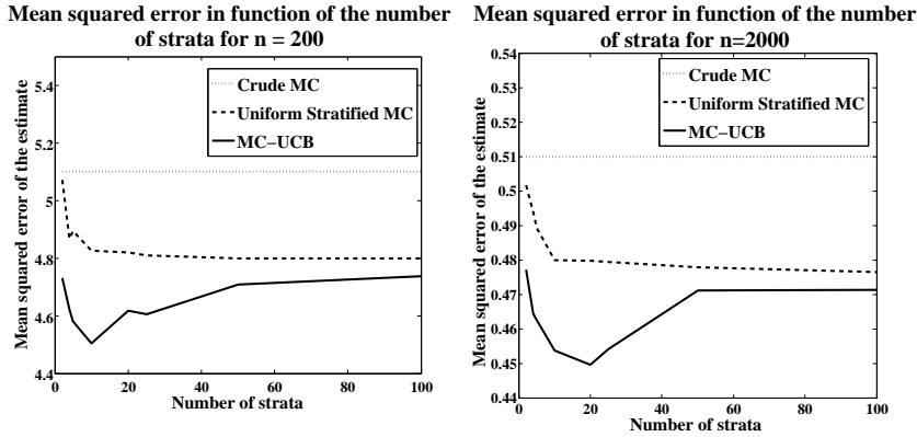
Fig. 2. Mean squared error for crude Monte-Carlo, uniform stratified sampling and MC-UCB, for different number of strata, for (Left:) n=200 and (Right:) n=2000 .
